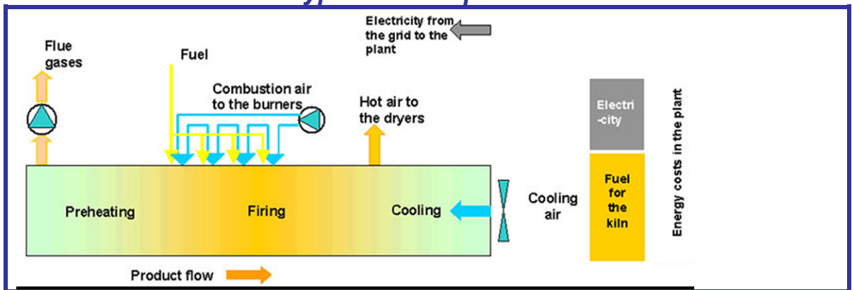
Typical Kiln Operation
