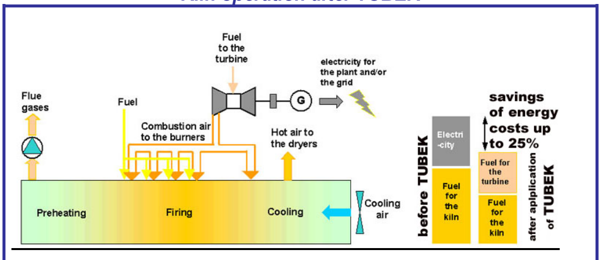
Kiln operation after TUBEK
