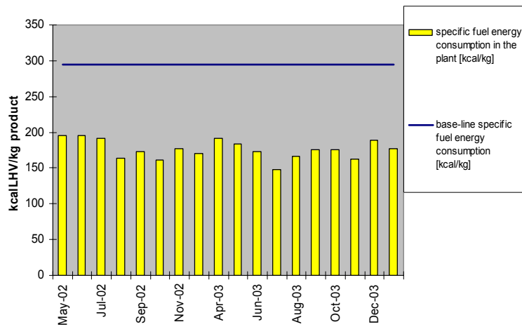
specific fuel energy consumption in the plant before and after TUBEK application -turbine set excluded-
